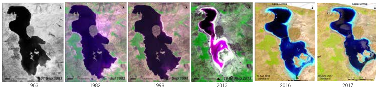
Changes in the surface area of Lake Urmia (1963-2017) Source: UNEP
