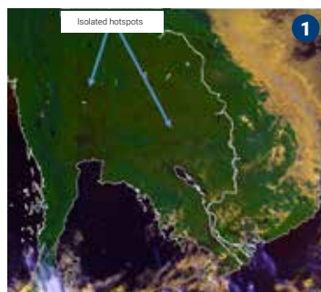
NOAA-19 Satellite 23 December 2017 0842 UTC
